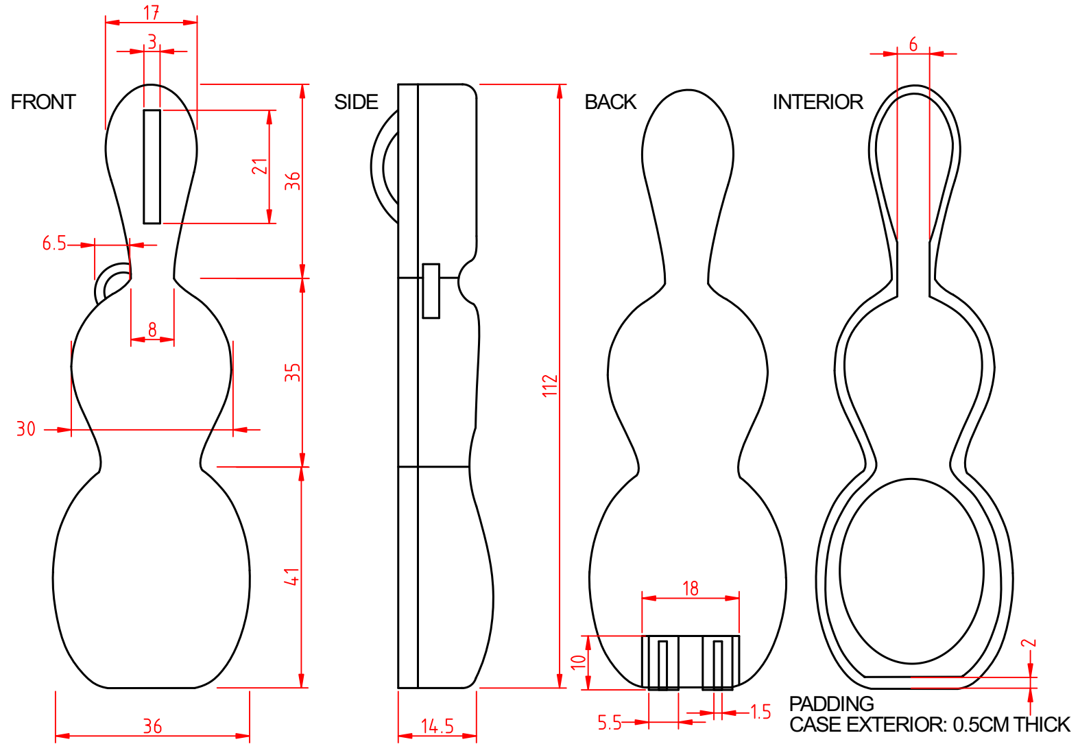
Sotendo Case Hard Cello Case CC-2010 Material: Fibreglass 3 metal catches Dimensions in cm, may vary slightly
